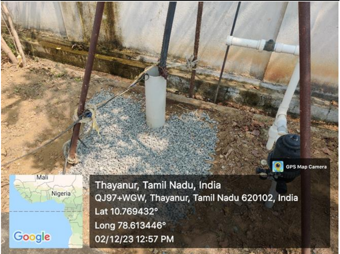
Fig. 7.1.4.3 Borewell recharge system
